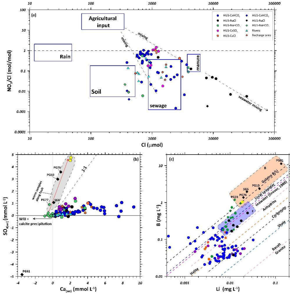
Figure 6 – (a) \text{NO}_3^-/\text{Cl} molar ratios versus \text{Cl} concentration (in \mu\text{mol} ) of the groundwater samples from Gioia Tauro Plain. In the diagram the representative fields of rain, agricultural, soil, sewage, and manure inputs, adapted from Torres-Martínez et al., 2021 , Awaleh et al., 2022 , Taussi et al., 2022 are reported. Binary plots (b) \text{Ca}_{(\text{wr})} vs. \text{SO}_{4(\text{wr})} and (c) \text{Li} vs. \text{B} showing the water samples from the Gioia Tauro Area. See the main text for figure details.
