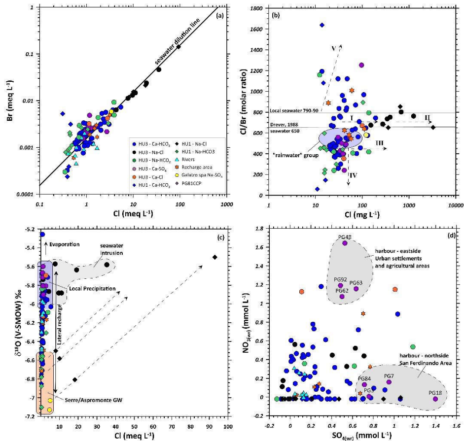
Figure 5 – Binary plots (a) Cl vs. Br, (b) Cl vs. Cl/Br, (c) \delta^{18}\text{O} vs. Cl and (d) \text{NO}_3(\text{wr}) vs. \text{SO}_4(\text{wr}) showing the water samples from the Gioia Tauro Area. See the main text for figure details.
