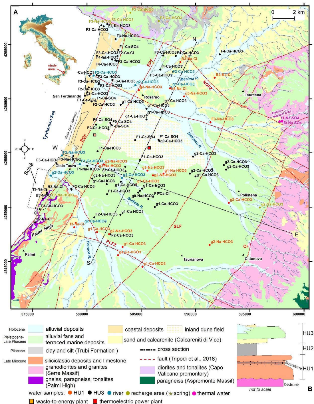
154 155 Figure 1 – (a) Simplified geological map of the Gioia Tauro area (modified after Cianflone et al., 2021 ) showing location and ID 156 ( Stuyfzand, 1986 ) of water samples (red symbols: deep aquifer; black symbols: shallow aquifer); (b) schematic stratigraphic column 157 (not to scale) showing the deep (HU1) and shallow (HU3) aquifers and the aquitard (HU2) recognized in the study area. NGFZ: 158 Nicotera-Gioiosa Fault Zone; PGF: Palmi-Gioia Tauro Fault; RPF: Rosarno-Palmi Fault; SLF: Sant'Eufemia-Laureana Fault; CF: 159 Cittanova Fault; PLFZ: Palmi-Locri Fault Zone. 160
