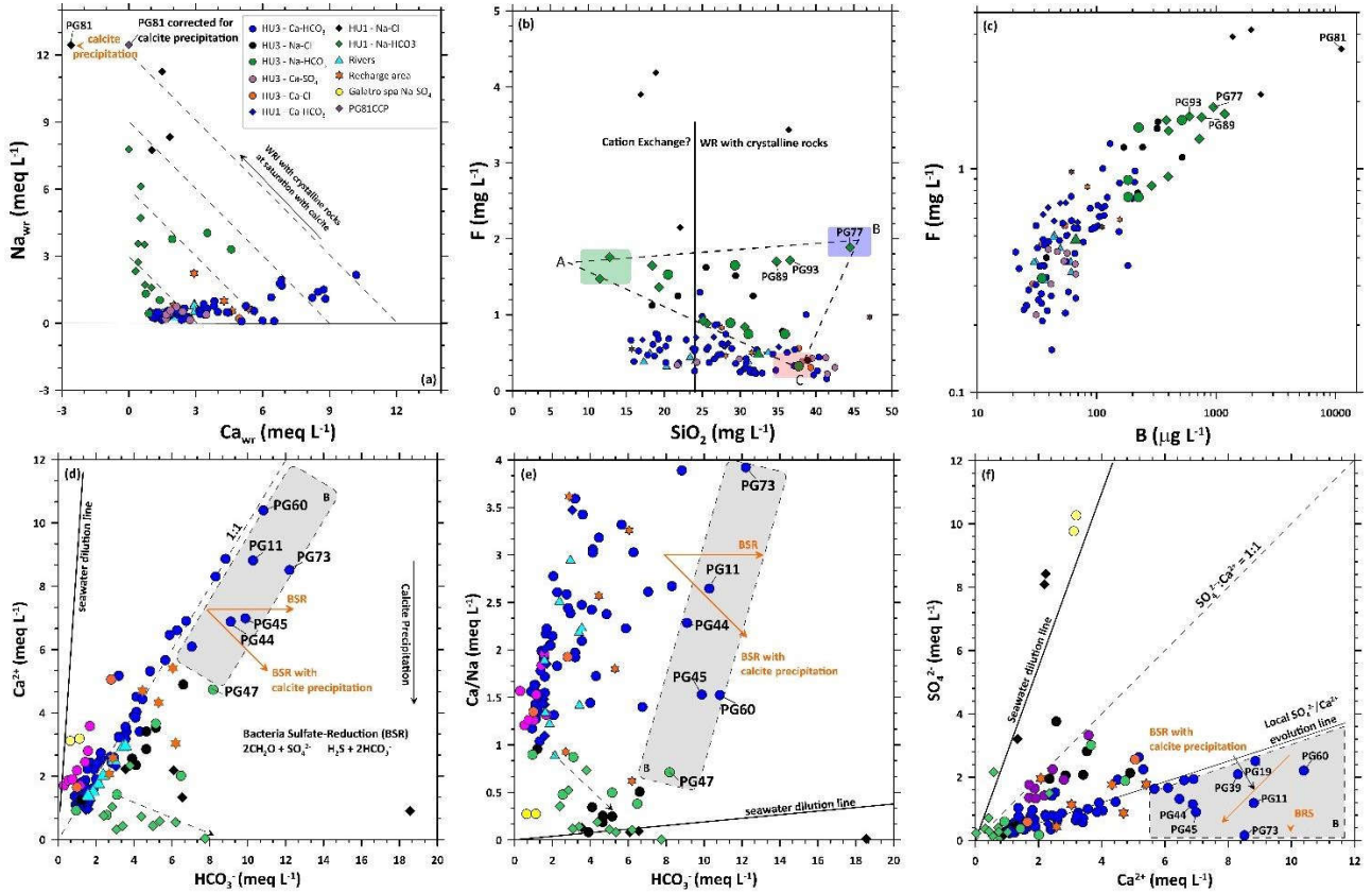
Figure 4 – Binary plots (a) \text{Ca}_w vs. \text{Na}_w , (b) \text{SiO}_2 vs. \text{F} , (c) \text{B} vs. \text{F} , (d) \text{HCO}_3^- vs. \text{Ca} , (e) \text{HCO}_3^- vs. \text{Ca/Na} and (f) \text{Ca} vs. \text{SO}_4 showing the water samples from the Gioia Tauro Area. BSR: Bacterial Sulphate Reduction. PG81CCP: corrected for calcite precipitation.
