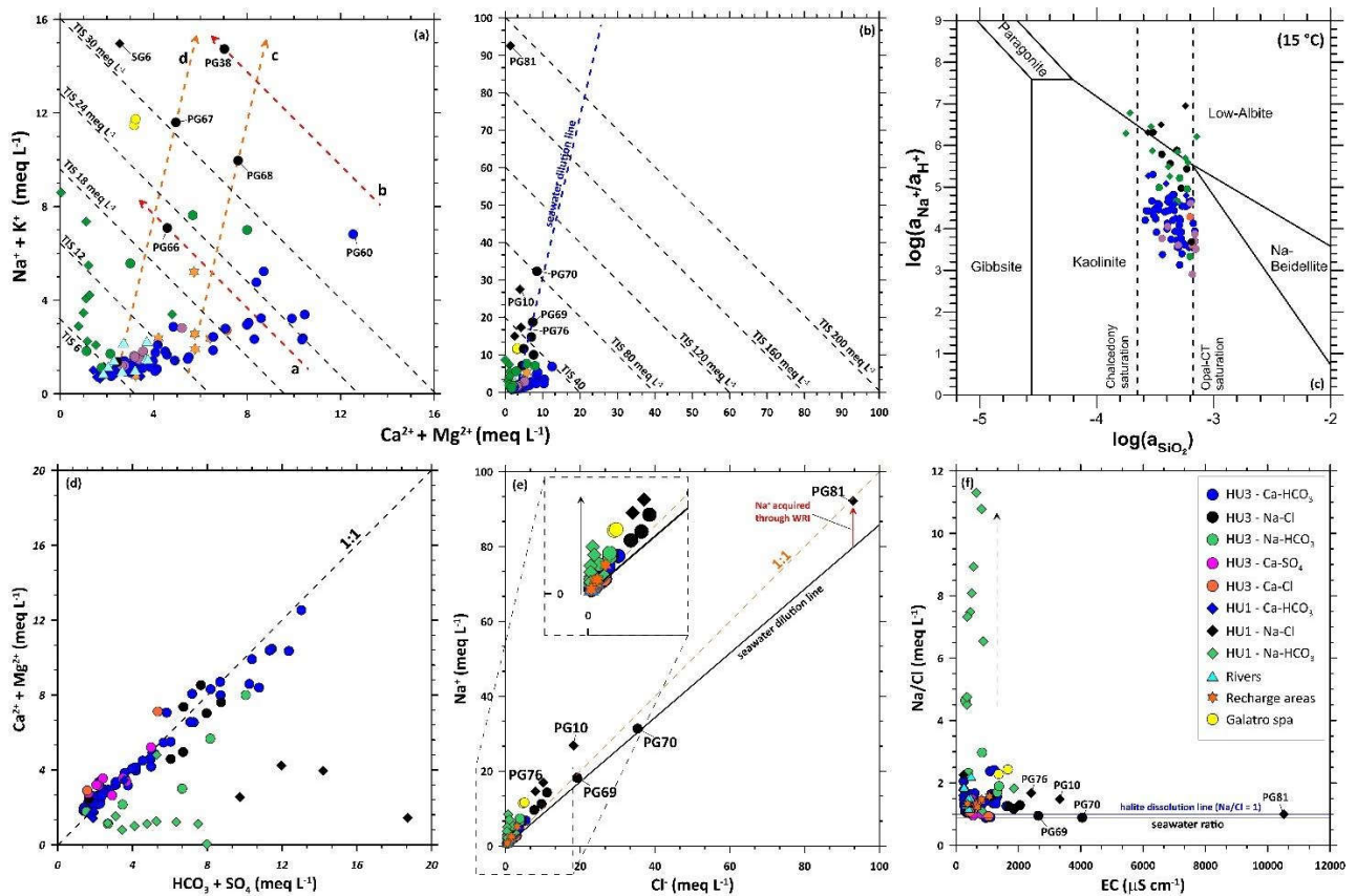
436 Figure 3 - Correlation diagram of (\text{Ca}^{2+} + \text{Mg}^{2+}) vs. (\text{Na}^+ + \text{K}^+) for (a) low and (b) high salinity samples from the GTP waters. Iso-salinity 437 lines are drawn for reference. Lines a, b, c, and d are discussed in the text. (c) Activity diagram (sensu Helgeson 1968) showing the 438 stability fields of low-albite, kaolinite, paragonite, gibbsite, Na-beidellite and saturation lines with respect to chalcedony and opal. 439 Binary plots (d) \text{Ca}^{2+} + \text{Mg}^{2+} vs. \text{HCO}_3^- + \text{SO}_4^{2-} , (e) \text{Cl}^- vs. \text{Na}^+ and (f) EC vs. \text{Na/Cl} showing the water samples from the Gioia Tauro 440 Area. 441 442
