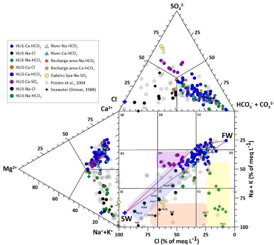
384 385 Figure 2 - Durov diagram showing the GTP water facies. Differences from the Ca-HCO 3 type are highlighted by colour shading, 386 namely: yellow for Na-HCO 3 of sectors B, C, D and F; orange for Na-HCO 3 (Cl) to Na-Cl of sector B; lilac for Na-Cl waters of sector 387 E (Scinà area); and purple for Ca-SO 4 and Ca-Cl waters of sector C. FW and SW represent freshwater and seawater, respectively.
