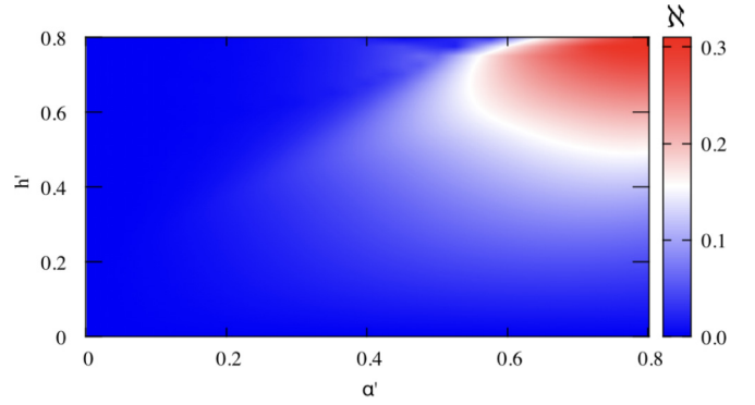
FIG. 7. Asymmetry of the critical current in the two direction for the four-region setup, calculated as a function of the dimensionless SOI \alpha' = \alpha m l_\omega / \hbar^2 and the dimensionless magnetization h' = h / E_\omega in the regions N_{SO} and N_F , respectively. For the numerical calculation we have set L_{SO1} = L_{F1} = 0.35l_\omega , and L_{SO2} = L_{F2} = 0.65l_\omega . The remaining parameters are the same as in Fig. 3.
