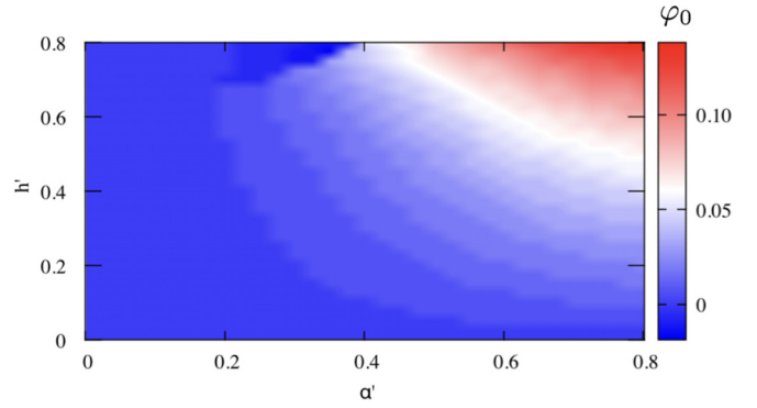
FIG. 4. Density plot of \varphi_0 as a function of the dimensionless SOI \alpha' = \alpha ml_\omega/\hbar^2 and the dimensionless magnetization h' = h/E_\omega in the regions N_{SO} and N_F , respectively. The remaining parameters are the same as in Fig. 3.
